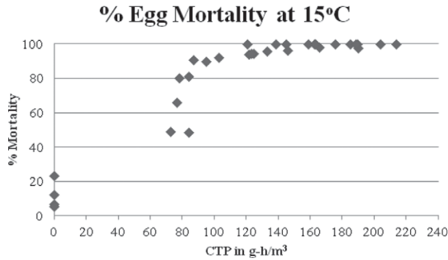
Fig. 4. Mortality of bedbug eggs after 7 d following a 24-h exposure to concentrations of SF, expressed as concentration \times time dosage ( \text{g}\cdot\text{h}/\text{m}^3 ) at 15^\circ\text{C} .
